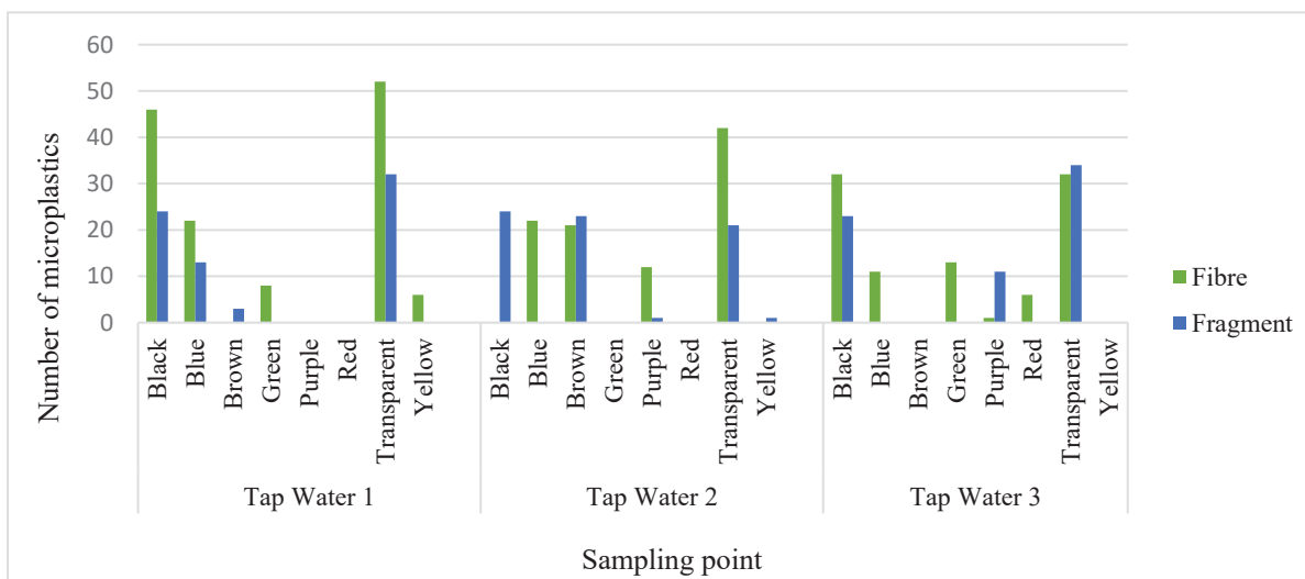
FIGURE 1. Microplastic abundance in the tap water samples
